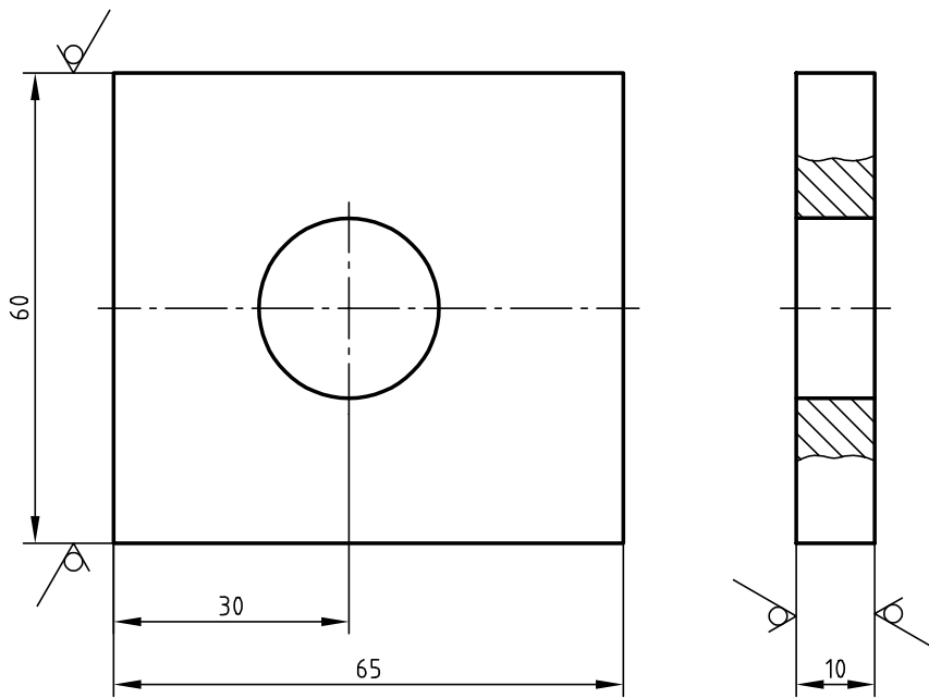
Skizze 1 \sqrt{Rz\ 16} ( \sqrt{\quad} )
