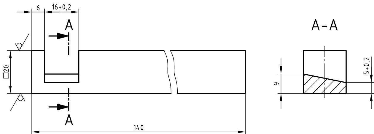
Skizze 3 \sqrt{Rz\ 16} ( \sqrt{\quad} )
