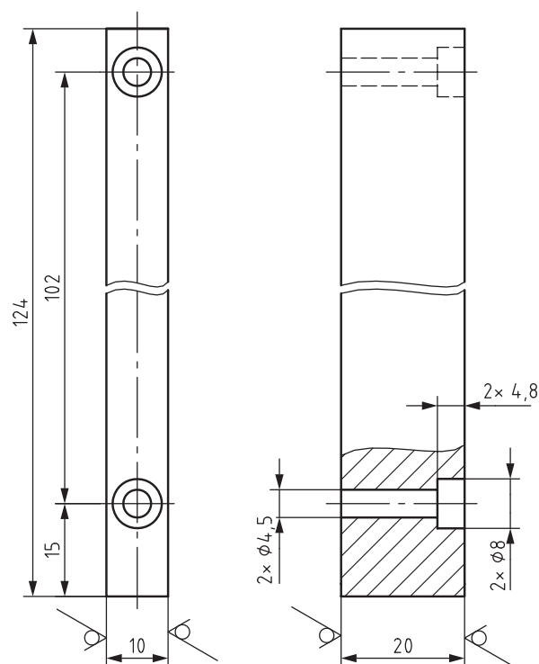
Skizze 8.5 \sqrt{Rz\ 16} (✓)
