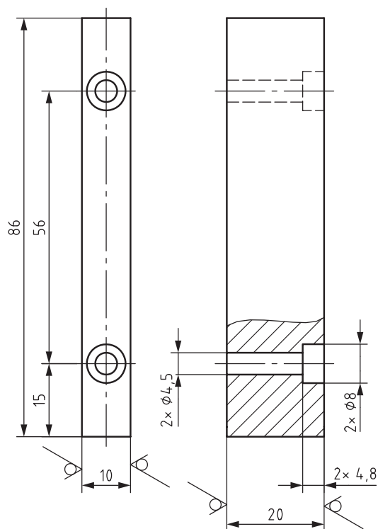
Skizze 8.3 \sqrt{Rz\ 16} (✓)
