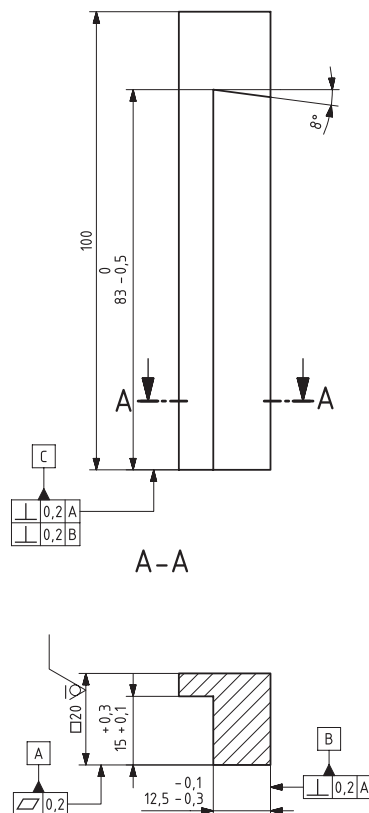
Skizze 7 \sqrt{Rz\ 16} ( \sqrt{\text{V}} )
